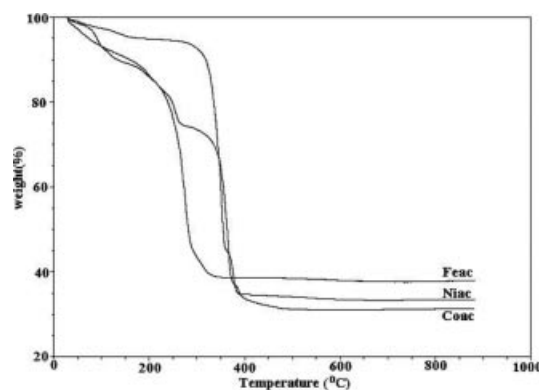
Figure 1. The TGA curve of Fe, Co, and Ni acetates.
